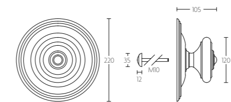
PB220
