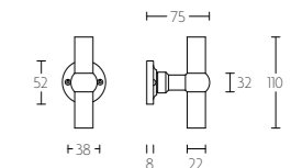
FV22D
