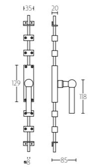
K-FVL125
